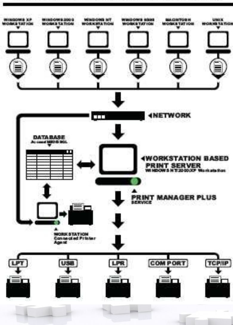
Print Manager Plus - WorkGroup (Peer-to-Peer) Setup Schematic
